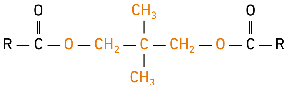
Figure 2. Polyol ester.
