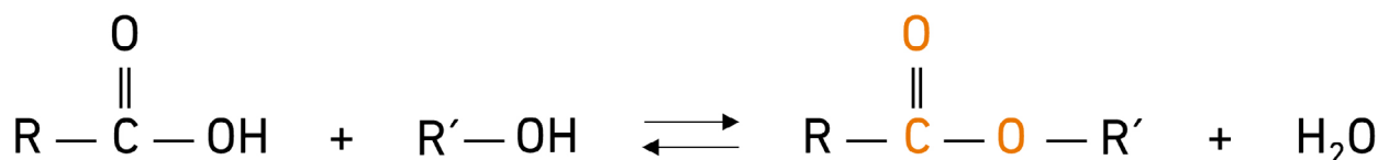
Figure 1. The esterification reaction
